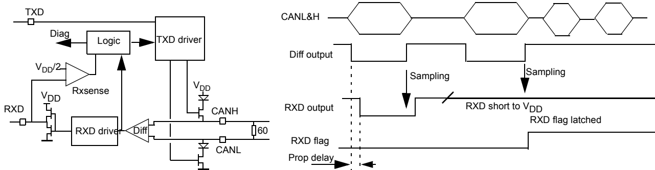
Figure 41. RXD Path Simplified Schematic, RXD Short to V_{DD} Detection
